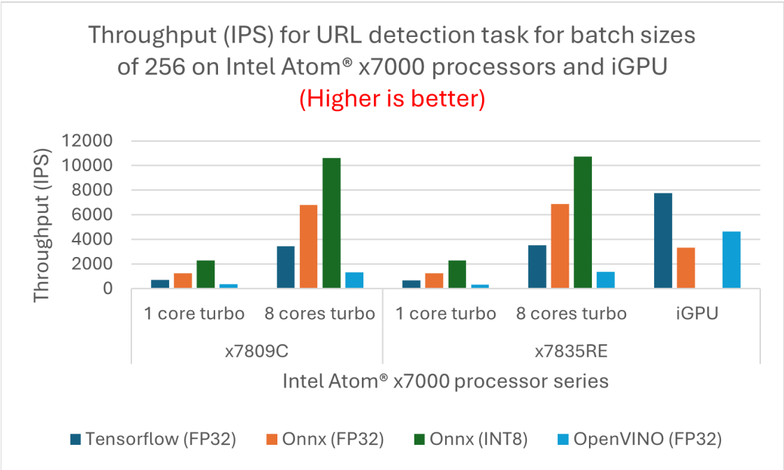
Figure 8. Throughput (IPS) for URL detection task for batch sizes of 256 on Intel Atom® x7000 processors on iGPU
