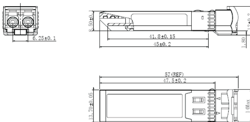
SL-SFP-1G-LX
