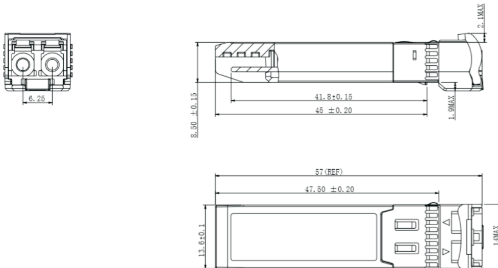
SL-SFP+10G-LR
